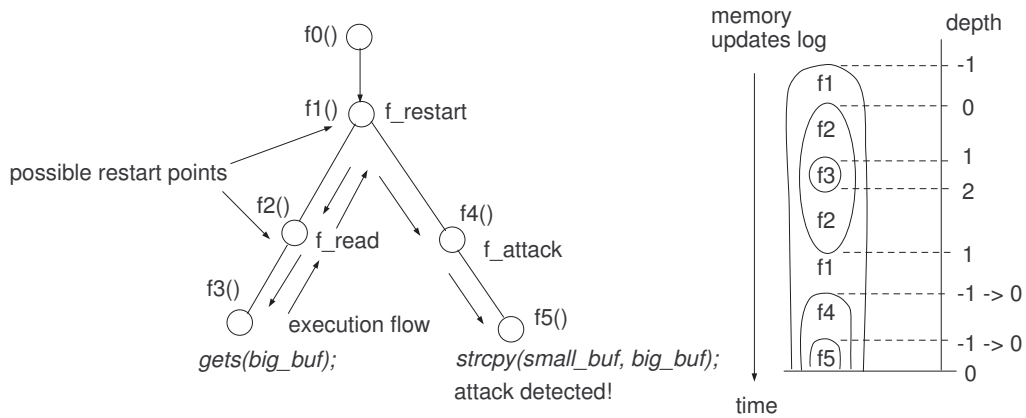
Figure 3. An example illustrating how to identify the least common dynamic ancestor in the function call graph and use it as the restart point. The right-hand side shows the memory updates log where f1–f5 are the same functions as those on the left-hand side. The ovals correspond to function boundaries. The depth values are the values of depth variable that is defined in Figure 4.
